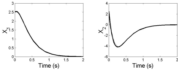
Fig. 1. Time responses of x_1 and x_2 under the feedback linearization control when \hat{\theta}(0) = 0.8
