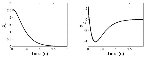
Fig. 2. Time responses of x_1 and x_2 under the feedback linearization control when \hat{\theta}(0) = 1.2
