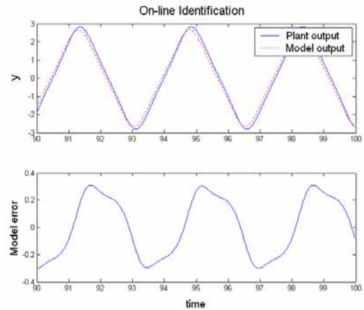
Fig. 4 The on-line ID of The Duffing system.
