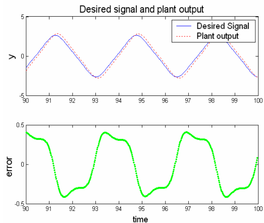
Fig. 5 The control result for Duffing system.
