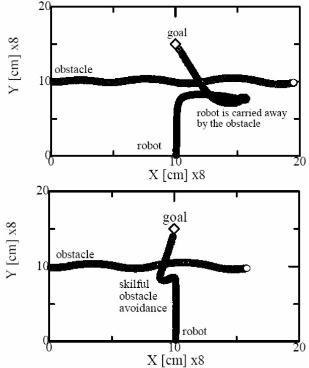
Fig 4 Experimental results of collision avoidance (conventional (upper) & proposed (lower) method)
