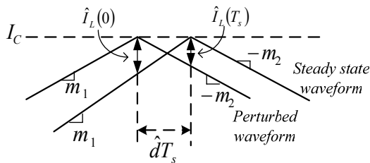
Fig. 8 Expanded view of steady state and perturbed inductor current magnitude waveform near peak value.
