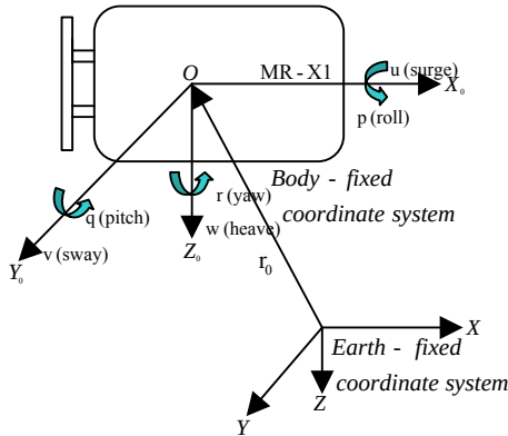
Fig.2 Coordinate system of 'MR-X1'
