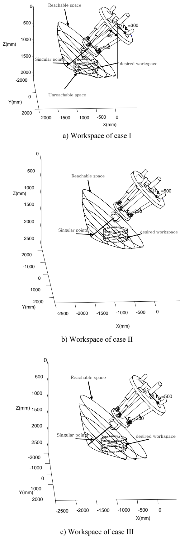
Fig. 3 Results of workspace analysis
