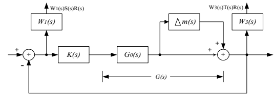
Fig. 5 Uncertainty model and the weighted sensitivity functions
