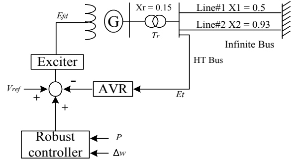
Fig. 2. System configuration using robust control.
