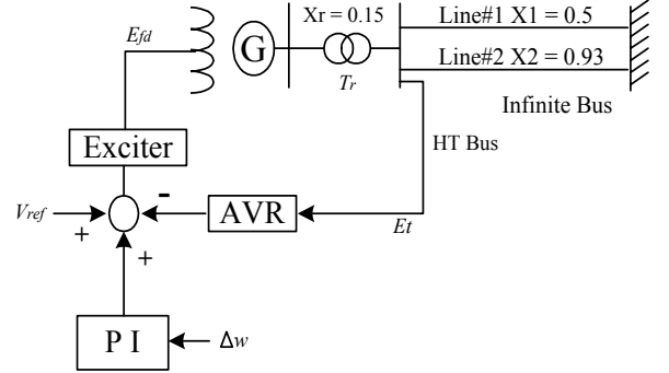
Fig 1. System configuration using the conventional PI control.
