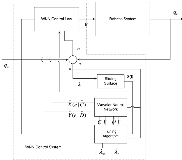
Fig. 3 WNNSMC scheme.
