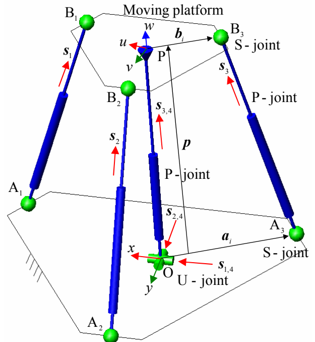
Fig. 4 Kinematic model of a Tricept parallel manipulator.
