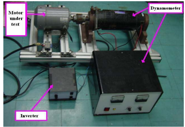
Figure 9. Overall System
