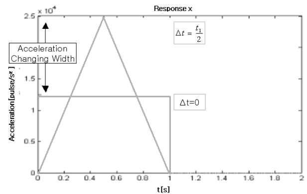
Fig. 4 Change of Acceleration according to Finite Jerk Duration
