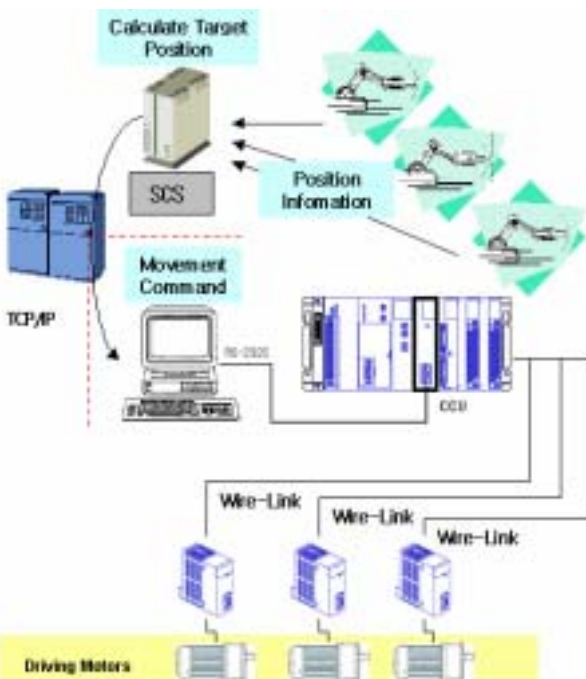
Fig. 11 Gantry crane control flow
