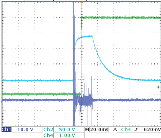
Fig. 9. Voltage Control
