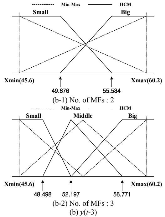
Fig. 4 Definition of initial membership functions of gas furnace process.
