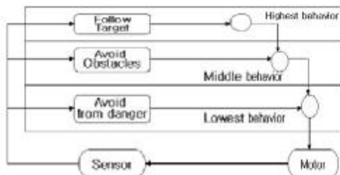
Fig. 9 Behavior-based fuzzy control architecture
