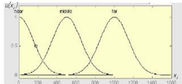
Fig. 6 Input membership function
