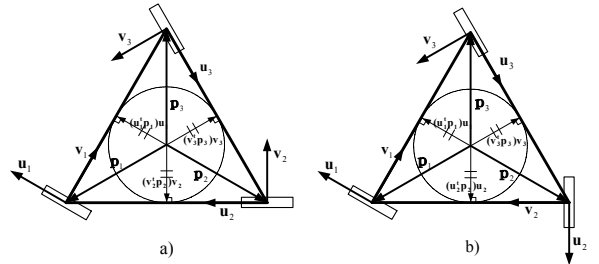
Fig. 4 With d=0 , isotropic configurations for NAG II: a) \Theta = \{\theta_1, \theta_2, \theta_3\} and b) \Theta = \{\varphi_1, \varphi_2, \varphi_3\} .
