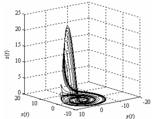
Fig. 2 Rossler attractor.
