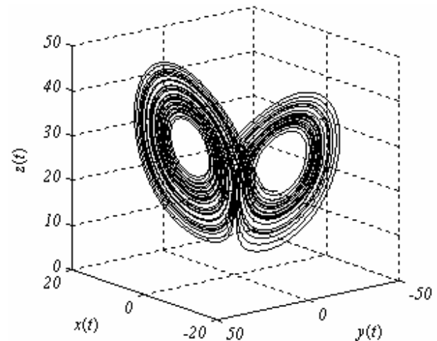
Fig. 1 Lorenz attractor.
