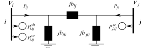
Fig. 3 The \pi -model of the UPFC-embedded line.
